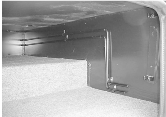
Slideout Crank Tools - typical
