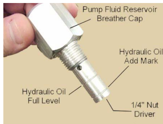
Hydraulic Fluid Dipstick HWH System Pump (F38J Model Only)
