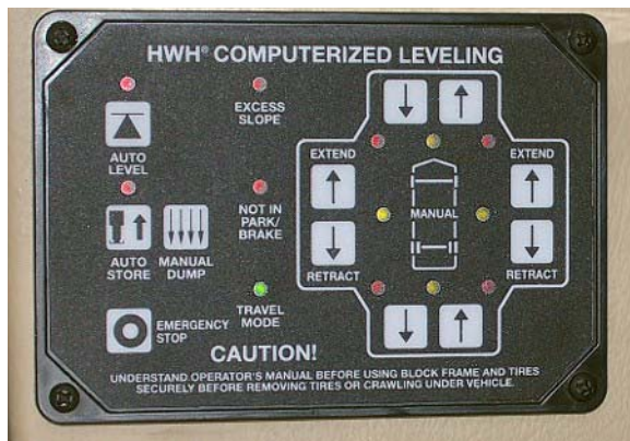
HWH Leveling Control Pad (F38J Model Only)
