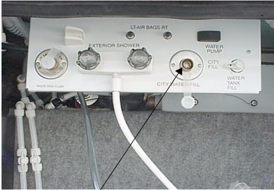
City Water Connection
