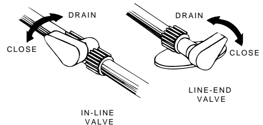
Waterline Drain Valves -Typical View
