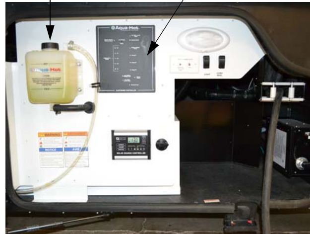
Hydronic Heating System (Located in driver side compartment) -Typical View
