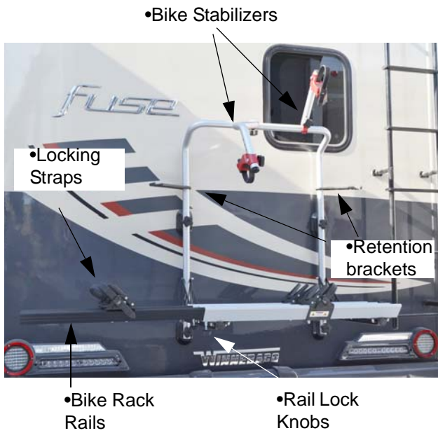
Bike Rack (shown in down position)
