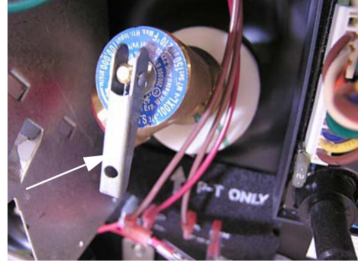
•Lift handle straight out to open P-T valve when water heater is cold. -Typical View
