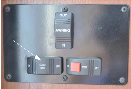
House/Coach Battery Disconnect Switch (Located near entrance door) -Typical View
