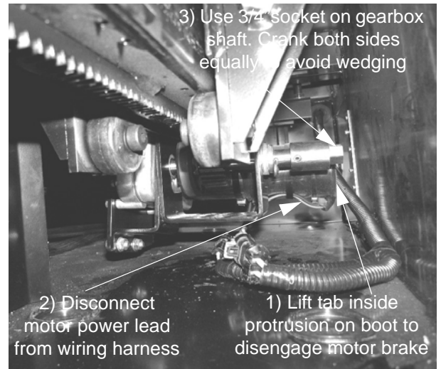
Slideout Motor/Gear Assembly (Located beneath each end of slideout room rail)
