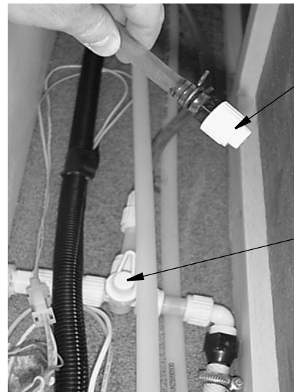
Winterization Valve -Typical View
