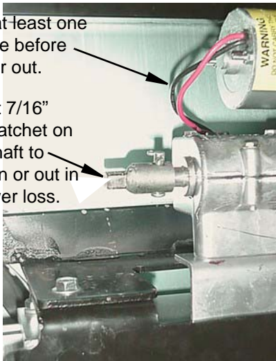
Front Slideout Room Motor/Gear Assembly (viewed from beneath coach)
