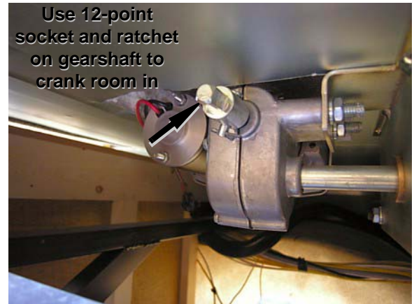
Rear Slideout Room Motor/Gear Assembly (view from access panel at foot of bed)
