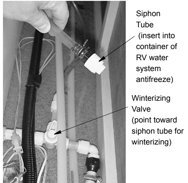
Winterization Valve (See Water Drain Valve Location chart for location on your coach)
