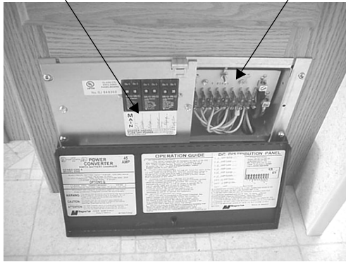
Load Center
