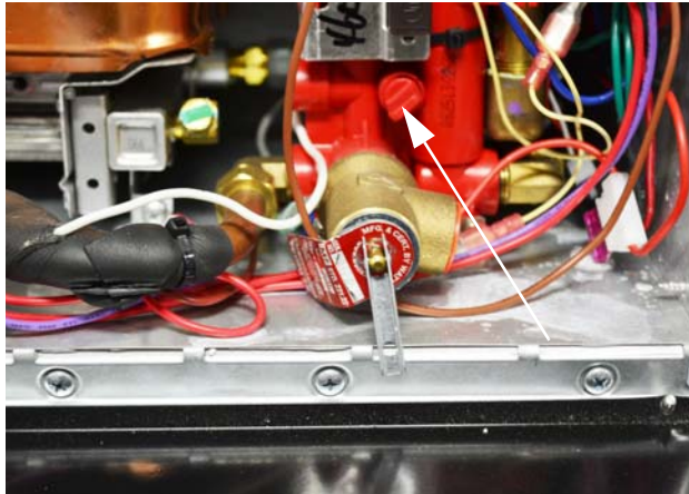
Modulating Valve
