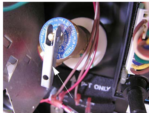
Pressure-Temperature Relief Valve (Lift handle only when water heater is cold)
