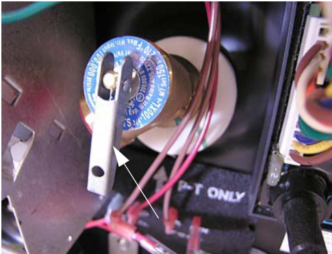
Pressure-Temperature Relief Valve (Lift handle only when water heater is cold)
