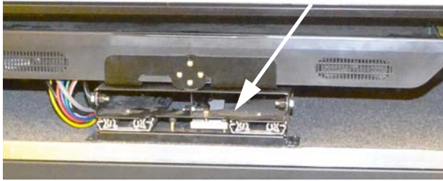
TV lock mechanism (Pull to the left to release)
